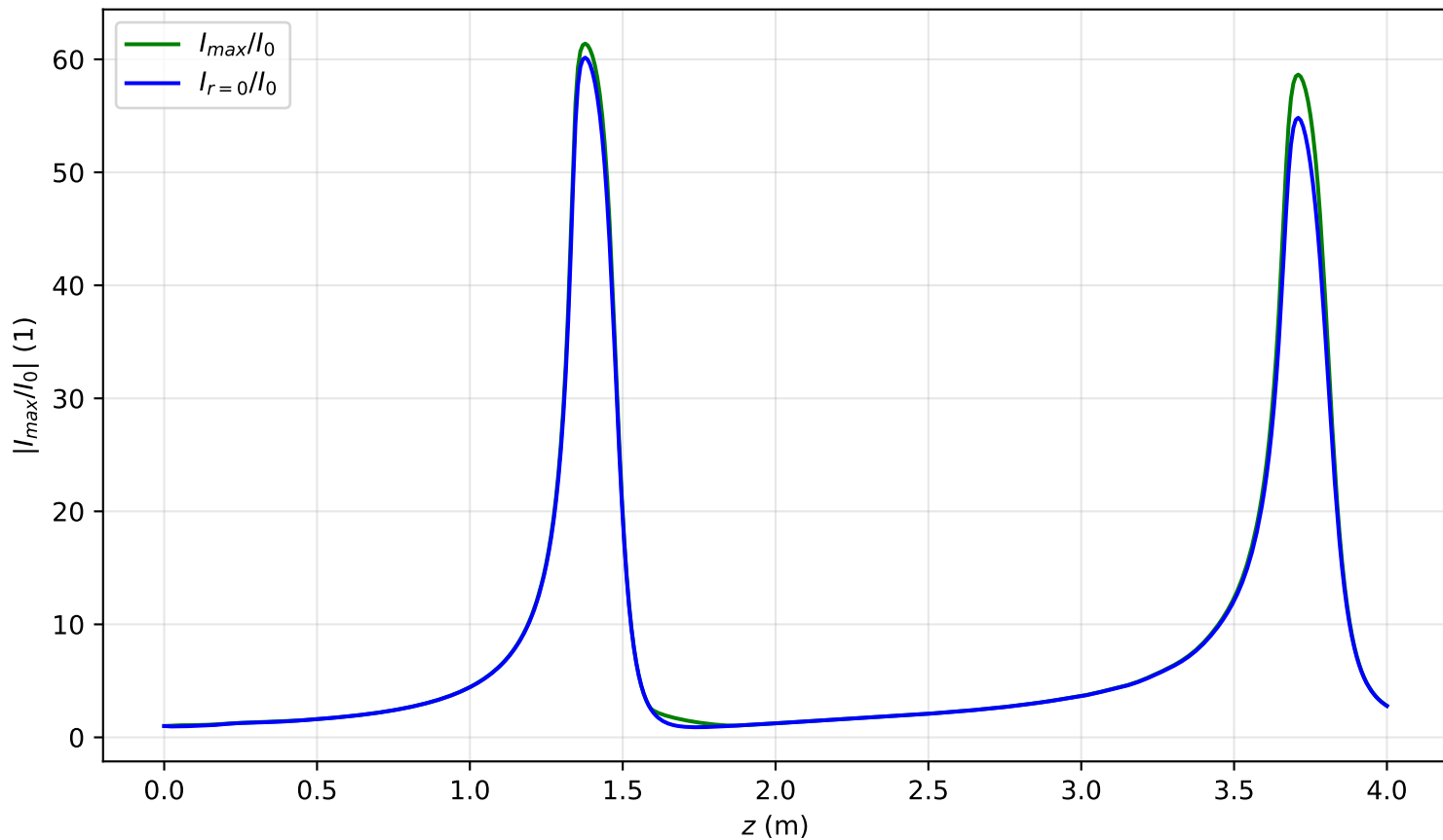
I_{max}(x = 0, y = 0, z)/I_0 , P_{in}=1.7P_{cr} , noisy input, artificial time
